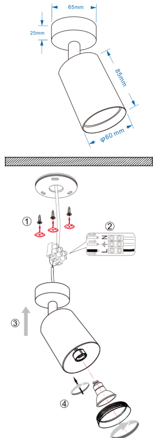
Item No.:TS5320 Finish: White
